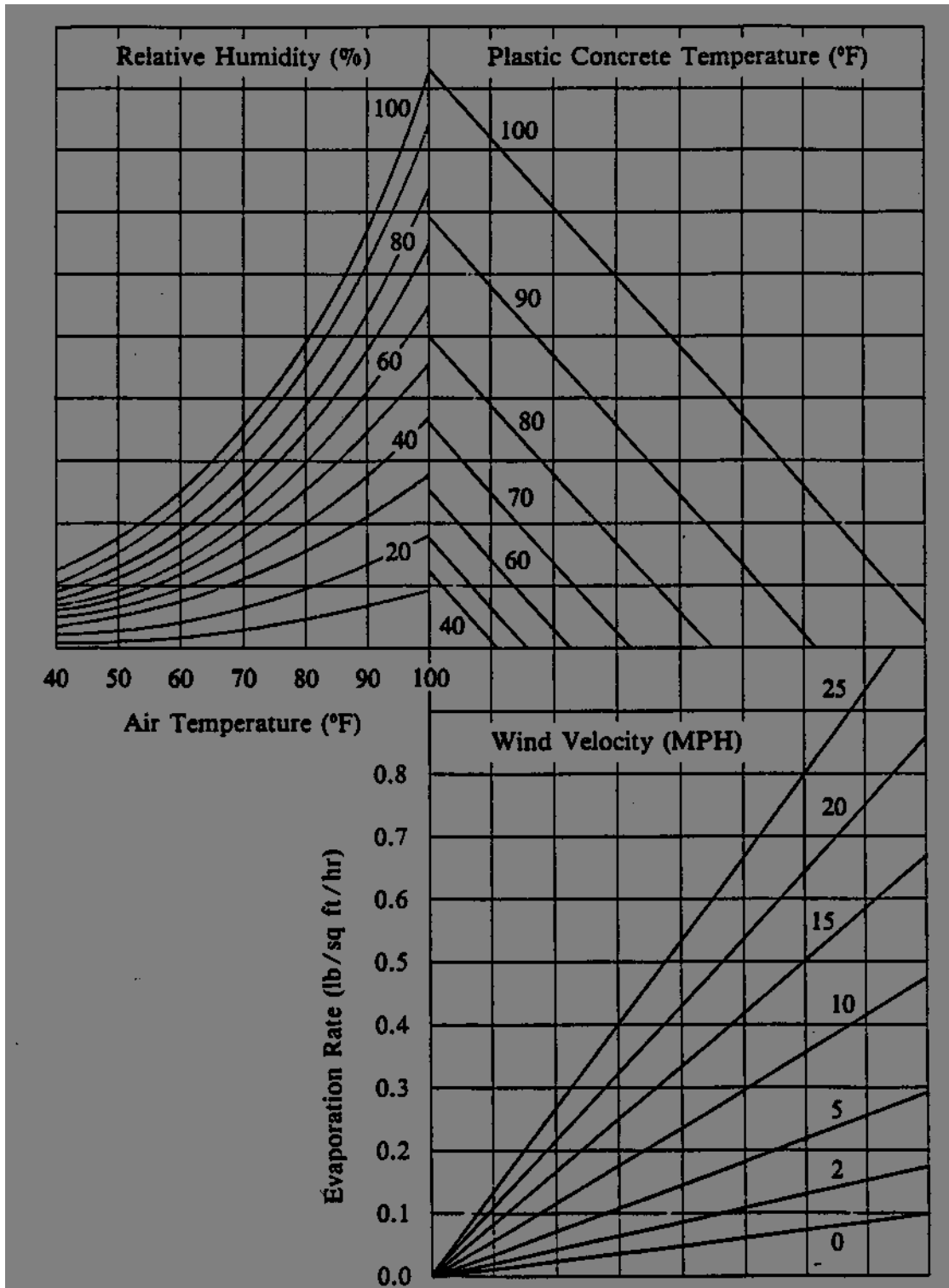
Chart 1 - Evaporation Rate (English)
